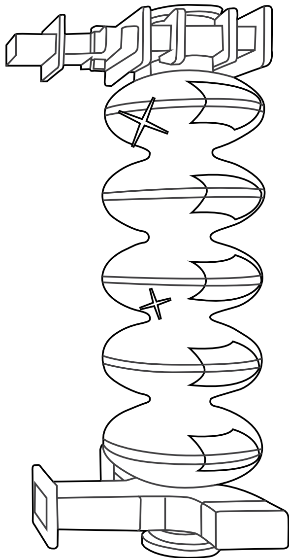
Original 5-Cell Cavity
